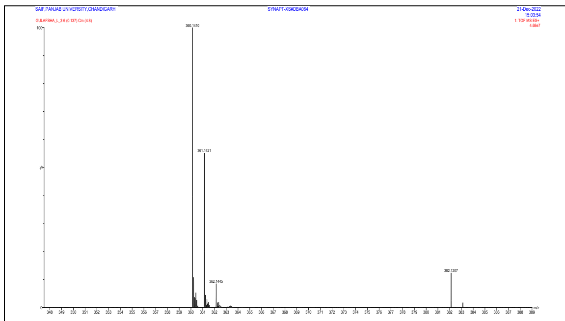
Figure 3. Mass Spectra of Schiff base ligand
