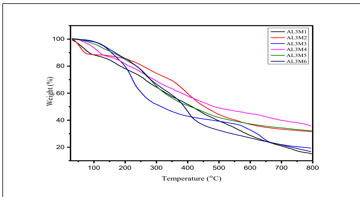
Figure 4. TGA spectra of transition metal complexes
