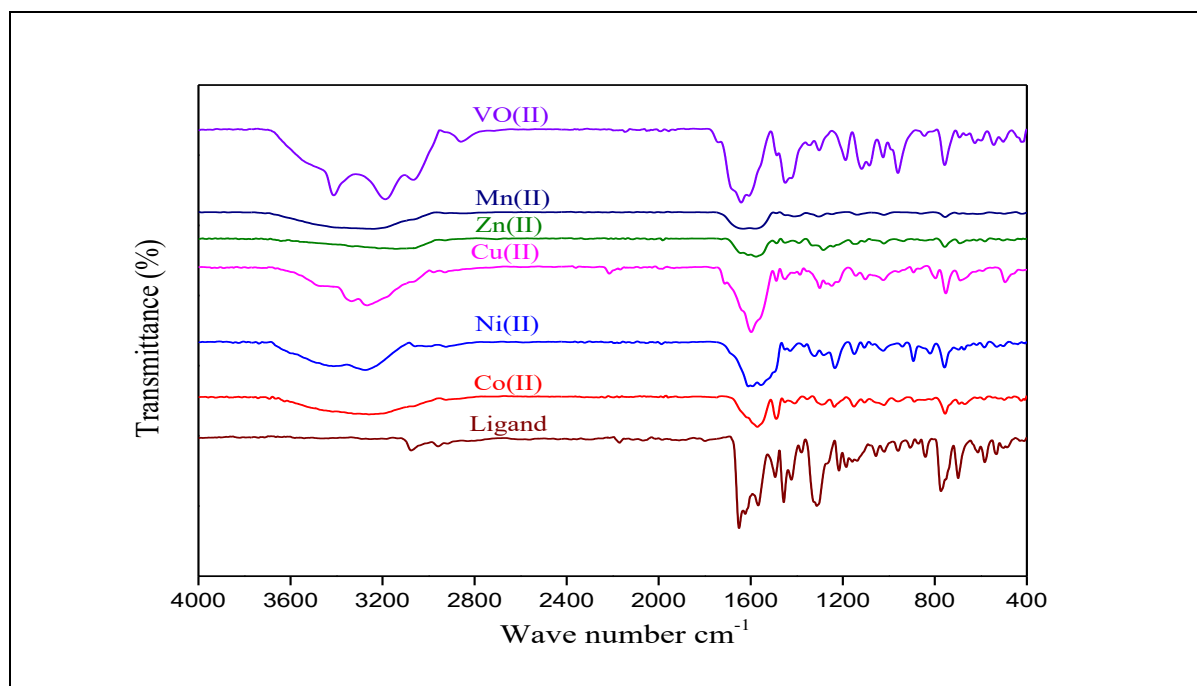
Figure 1. FT-IR Spectra of Schiff base ligand and transition metal complexes
