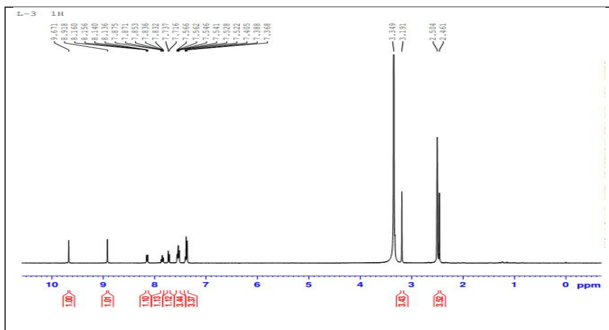
Figure 2. ^1\text{H} -NMR Spectra of Schiff base ligand
