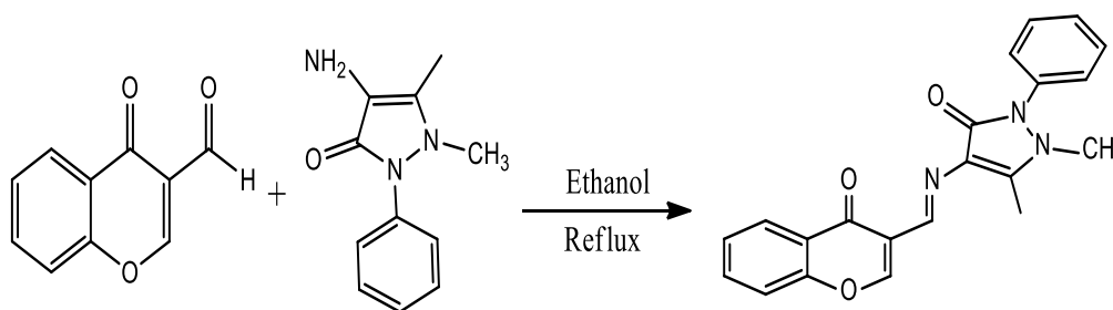
Scheme 1. Schematic route for the synthesis of Schiff base ligand
